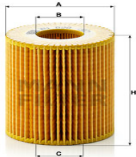
Oil Filter HU 820 x EM-10133
